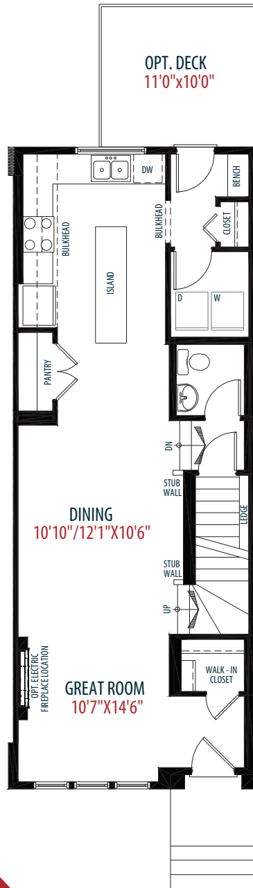
Main Floor 759 sq ft
